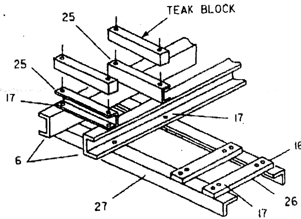
ERECTION OF SEALING ENDS AND SURGE DIVERTERS, STEELWORK
